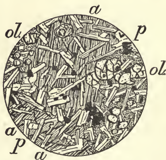
Fig. 39.—Basalt passing into Ophitic Dolerite. Tobermory, Mull. \times 25 . a , Augite, developed around the felspars in large ophitic crystals without defined outlines. In other places, to right and left, the hemicrystalline basaltic groundmass is seen in the interstices of the felspar mesh. ol , Olivine. p , Plagioclase; small prismatic habit characteristic of basalts. Magnetite also occurs.
